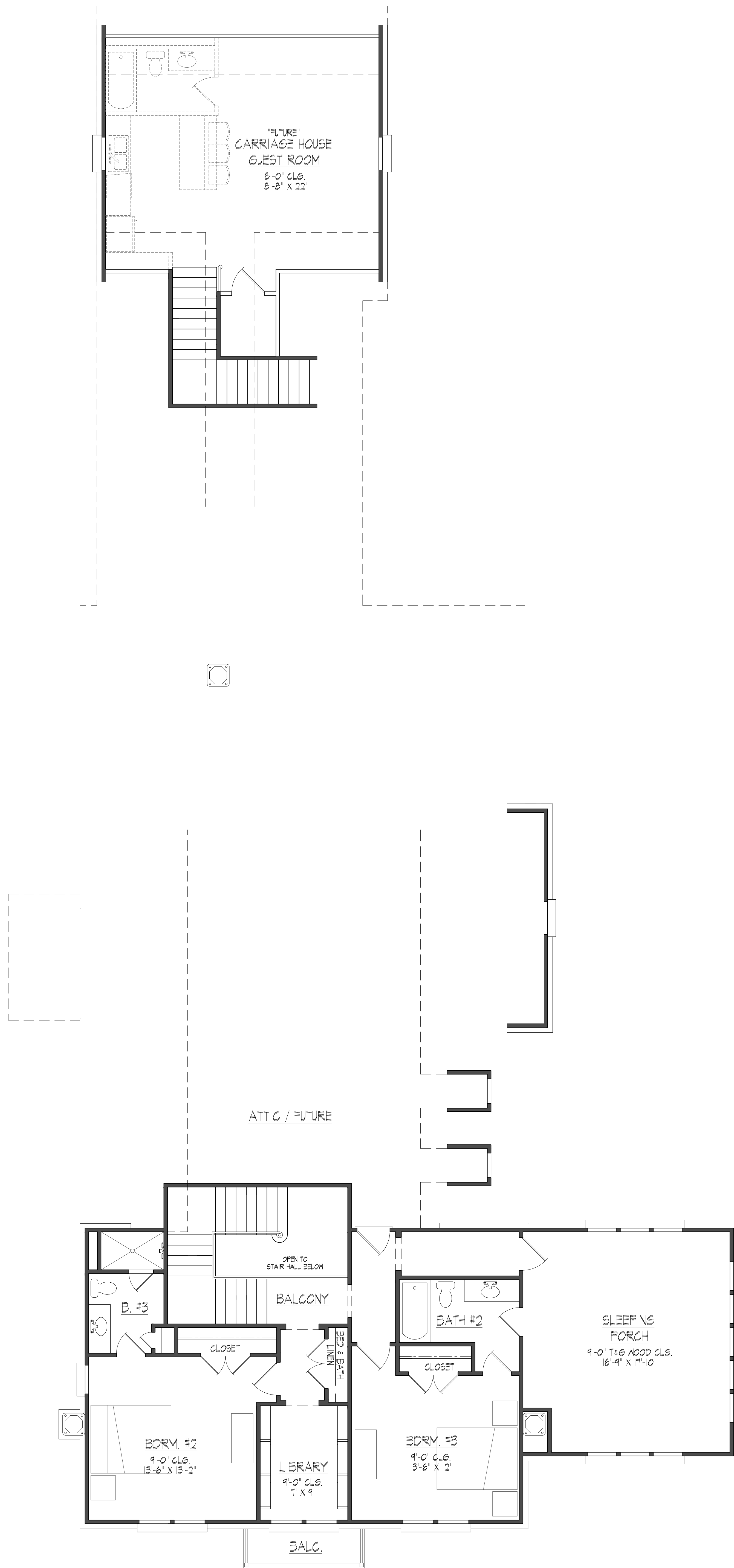
SECOND LEVEL FLOOR PLAN
