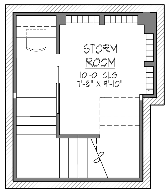
STORM ROOM LEVEL FLOOR PLAN
